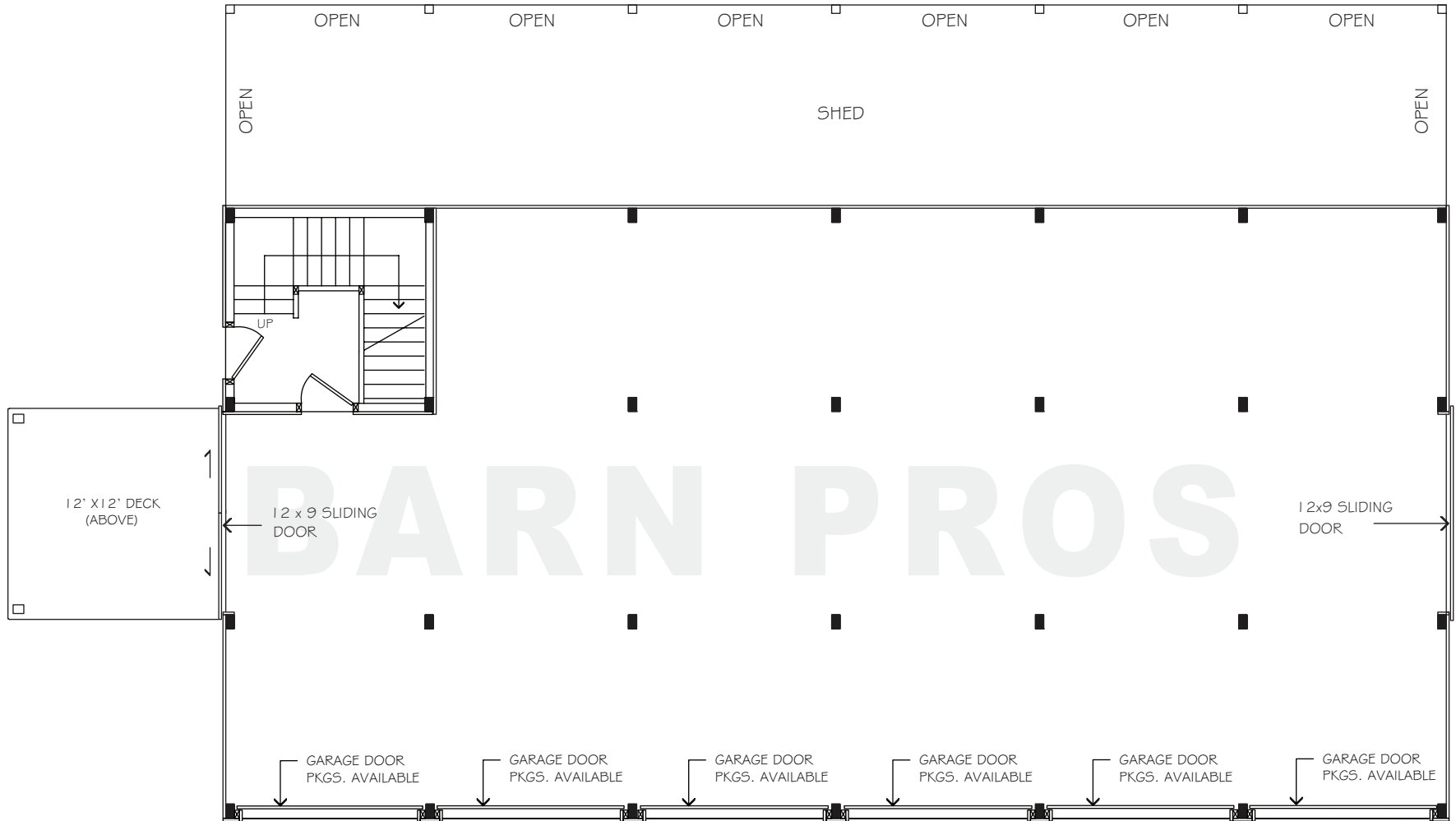
FLOORPLAN - LOWER
