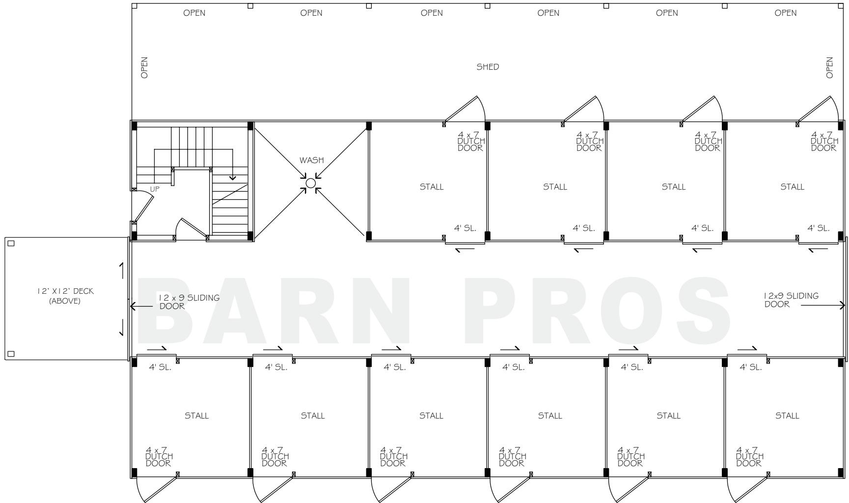
FLOORPLAN - LOWER
