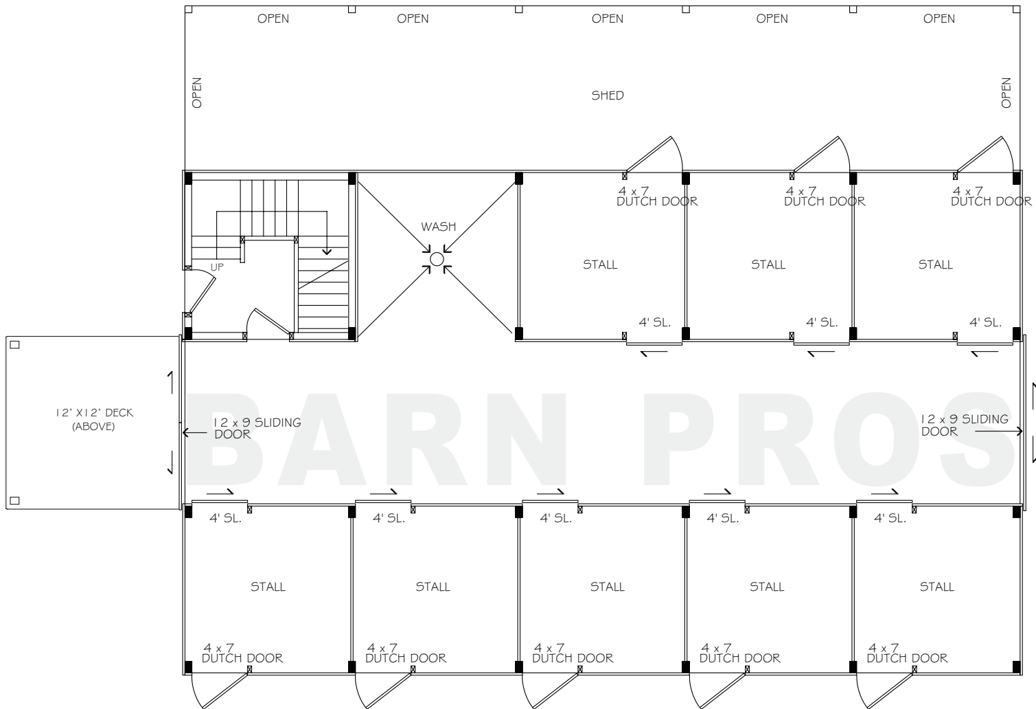
FLOORPLAN - LOWER
