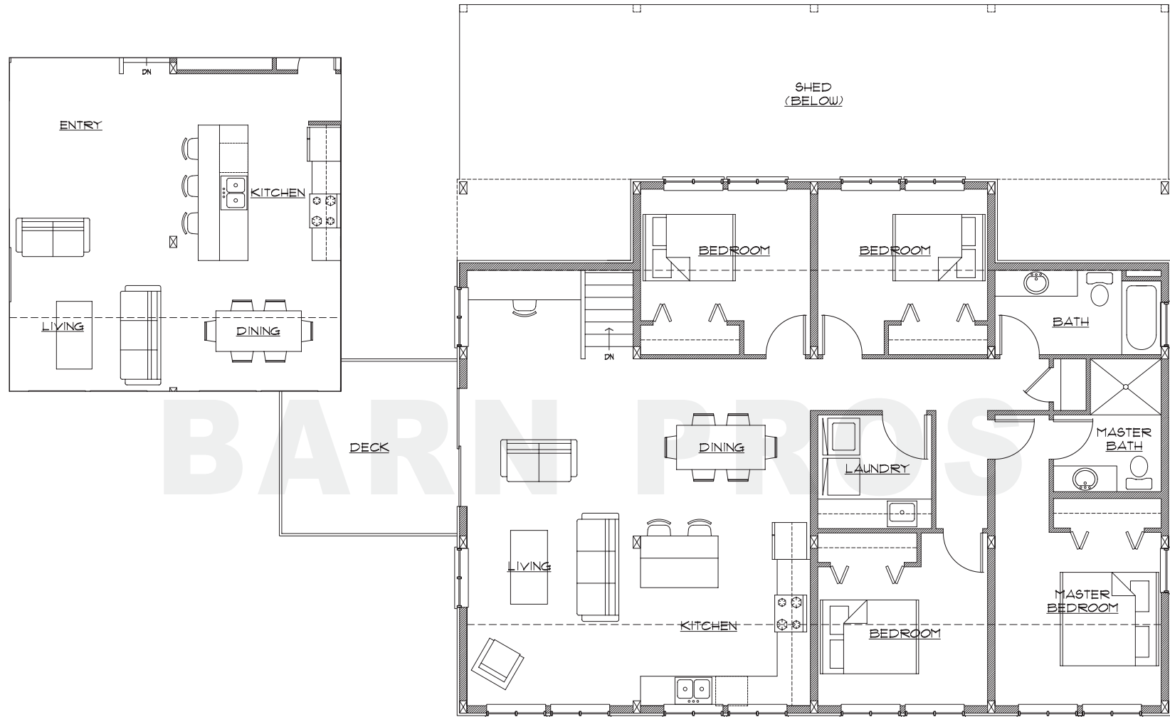
PROPOSED FLOORPLAN - UPPER Model B - Layout 1(right) & Layout 2(inset, upper left)
