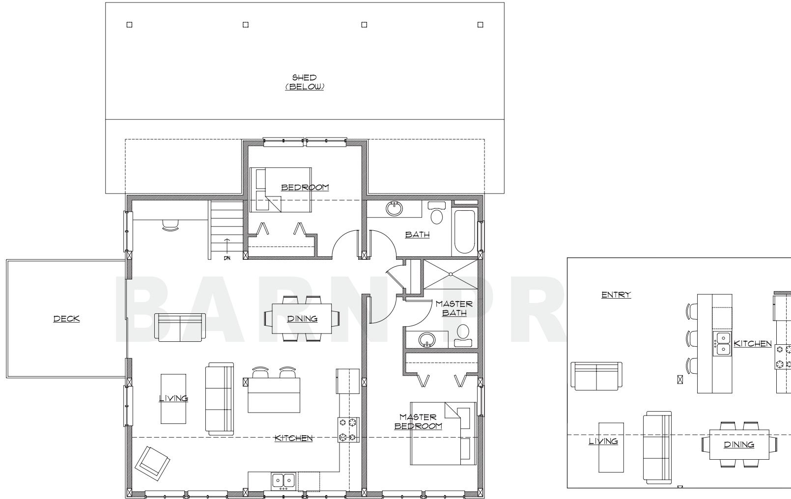
PROPOSED FLOORPLAN - UPPER Model B - Layout 1(left) & Layout 2(right)
