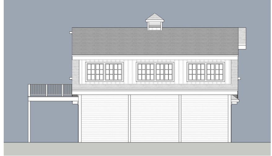
Side Elevation, Left
