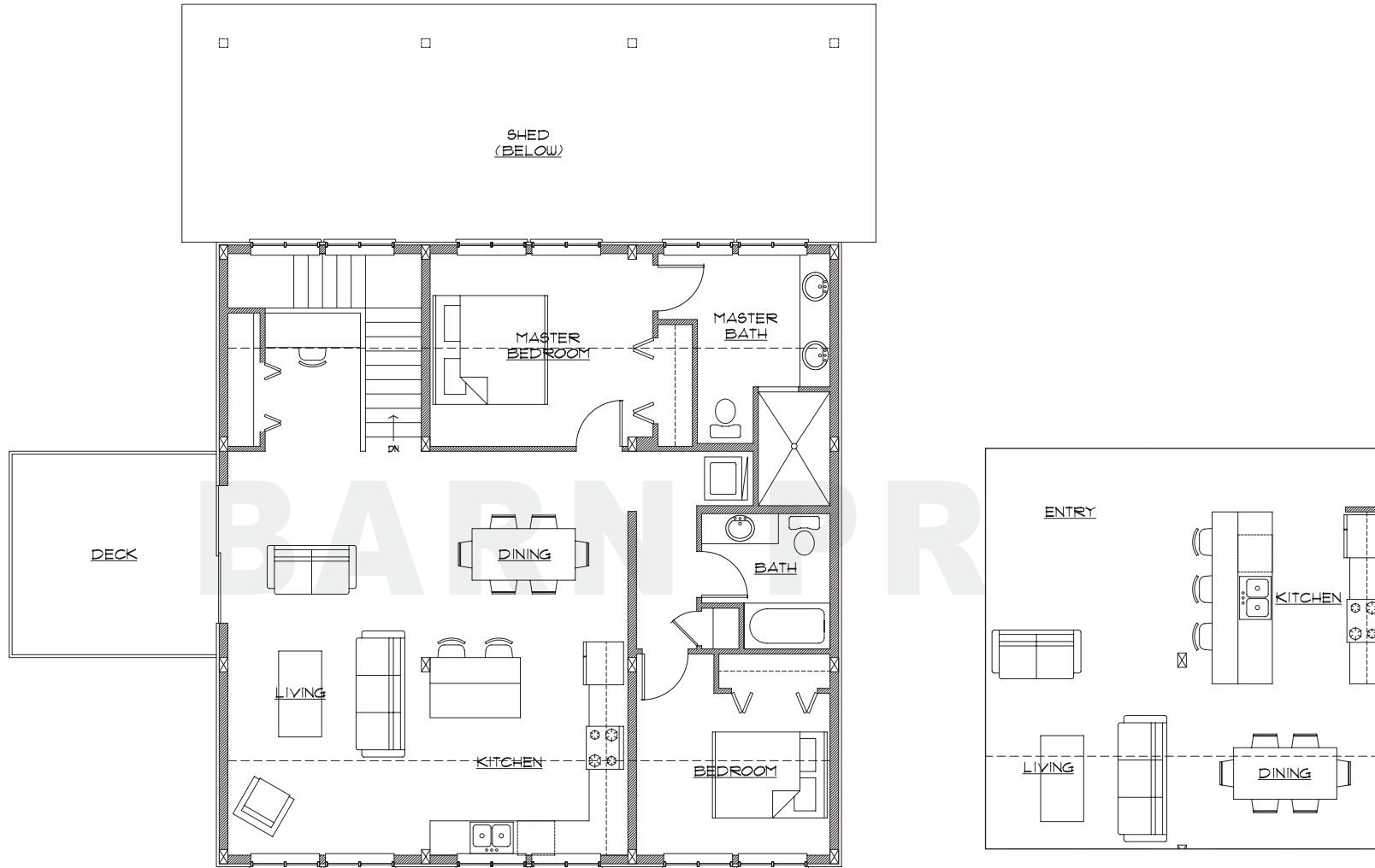
PROPOSED FLOORPLAN - UPPER Model D - Layout 1(left) & Layout 2(right)
