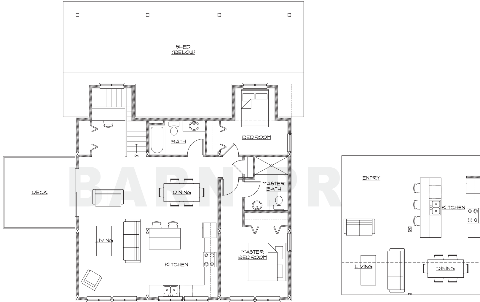
PROPOSED FLOORPLAN - UPPER Model A - Layout 1(left) & Layout 2(right)
