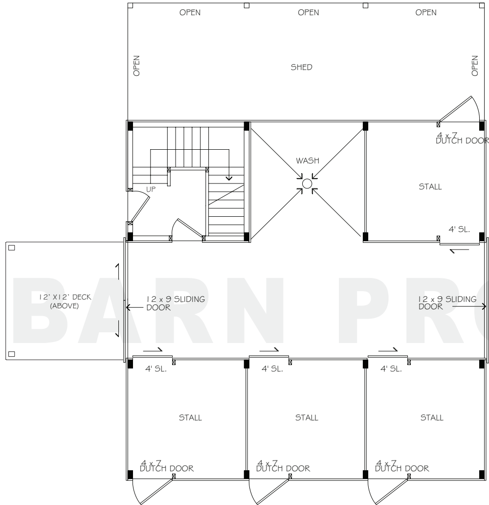
FLOORPLAN - LOWER
