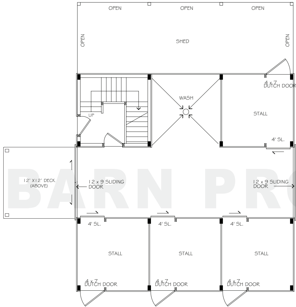
FLOORPLAN - LOWER
