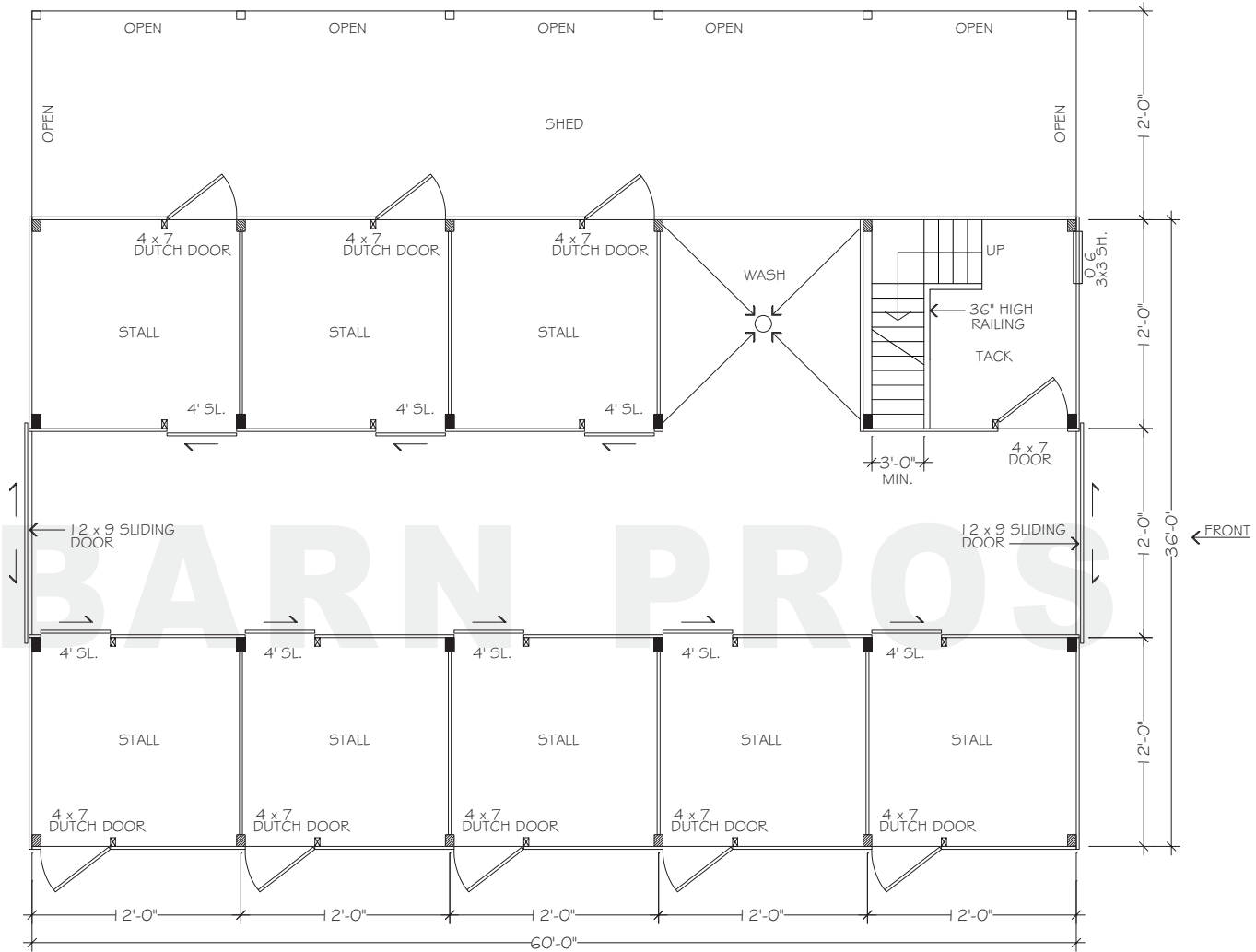
FLOORPLAN - LOWER
