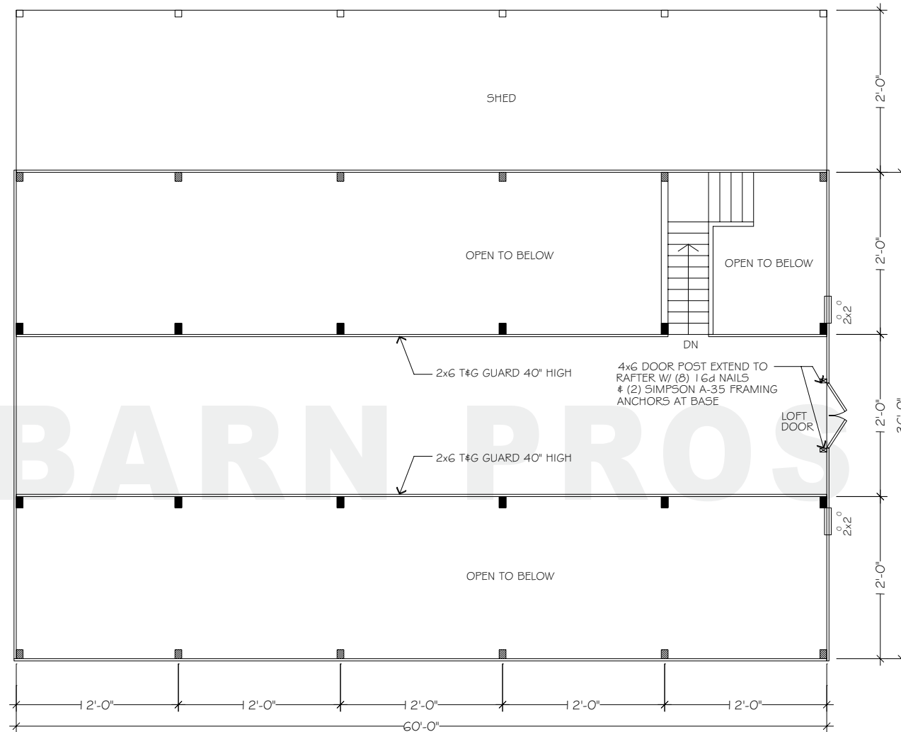
FLOORPLAN - UPPER
