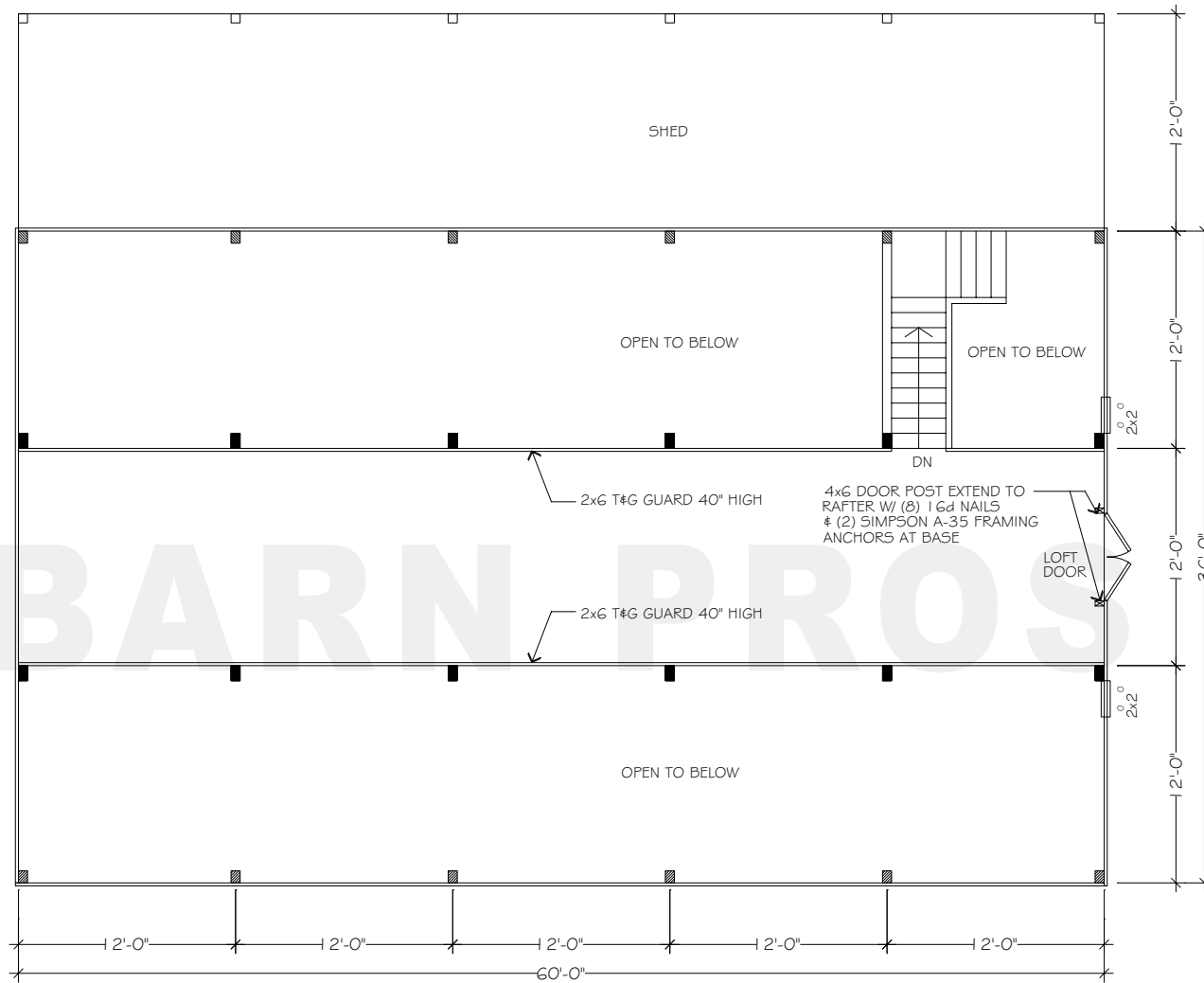
FLOORPLAN - UPPER
