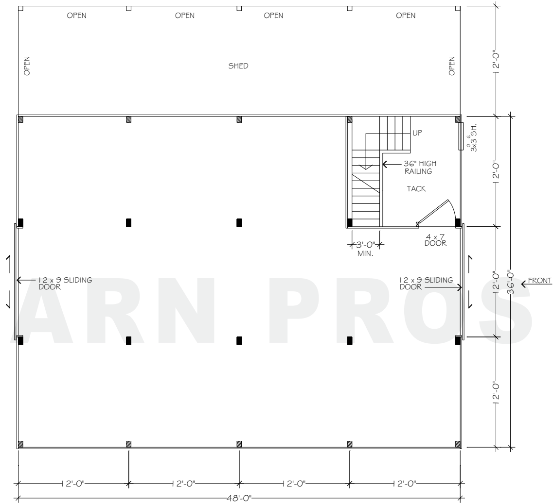
FLOORPLAN - LOWER
