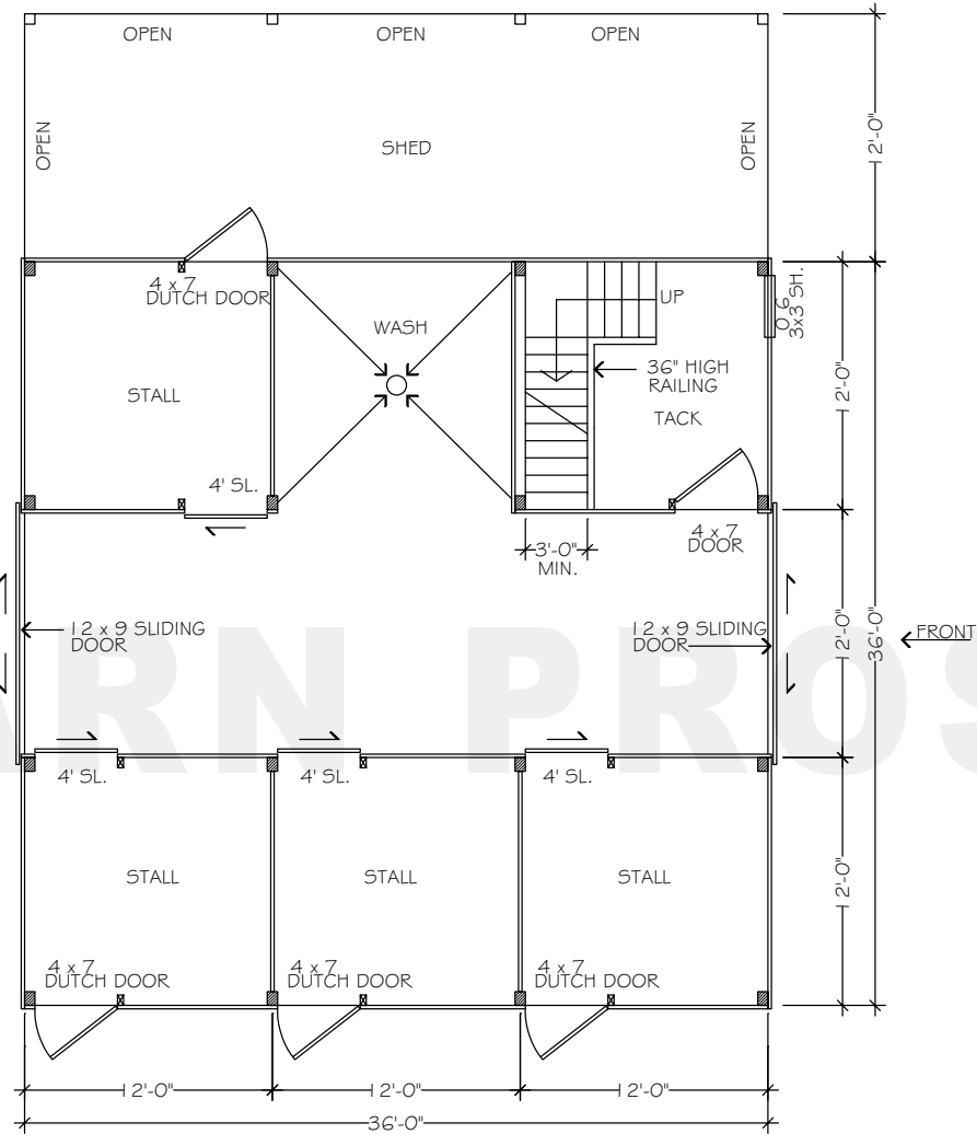
FLOORPLAN - LOWER
