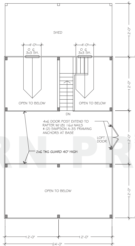
FLOORPLAN - UPPER
