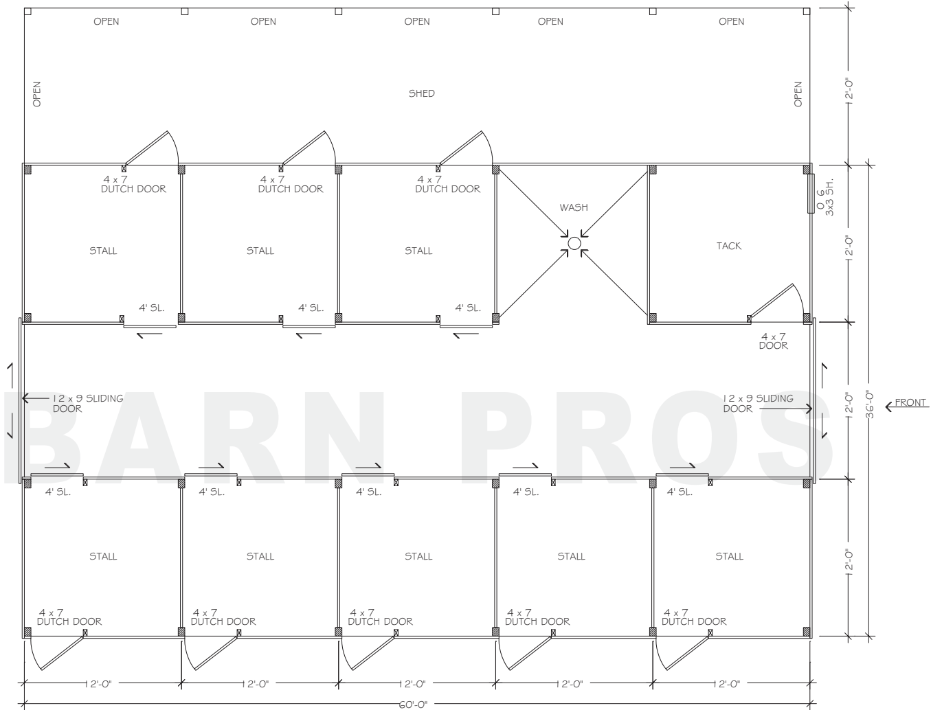
FLOORPLAN - LOWER
