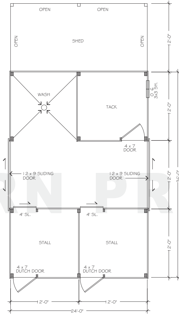
FLOORPLAN - LOWER
