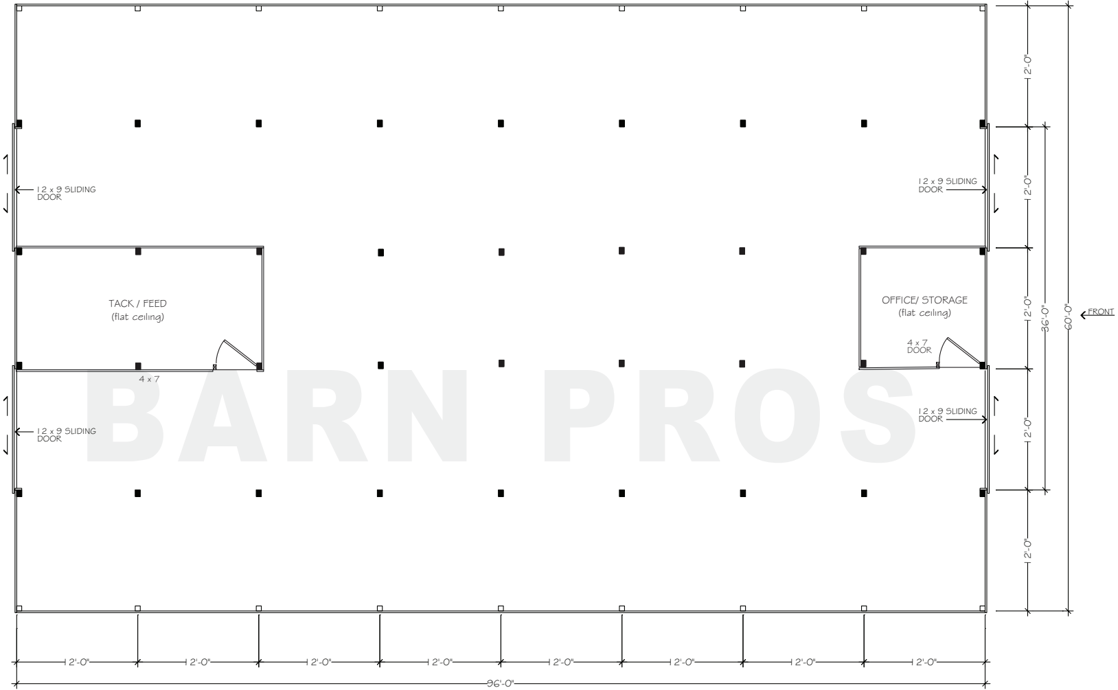
FLOORPLAN - LOWER
