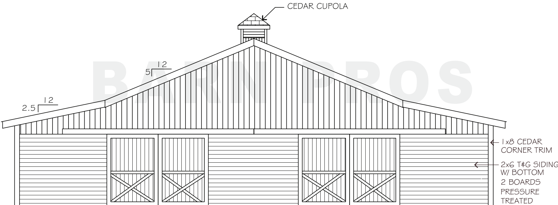
REAR ELEVATION
