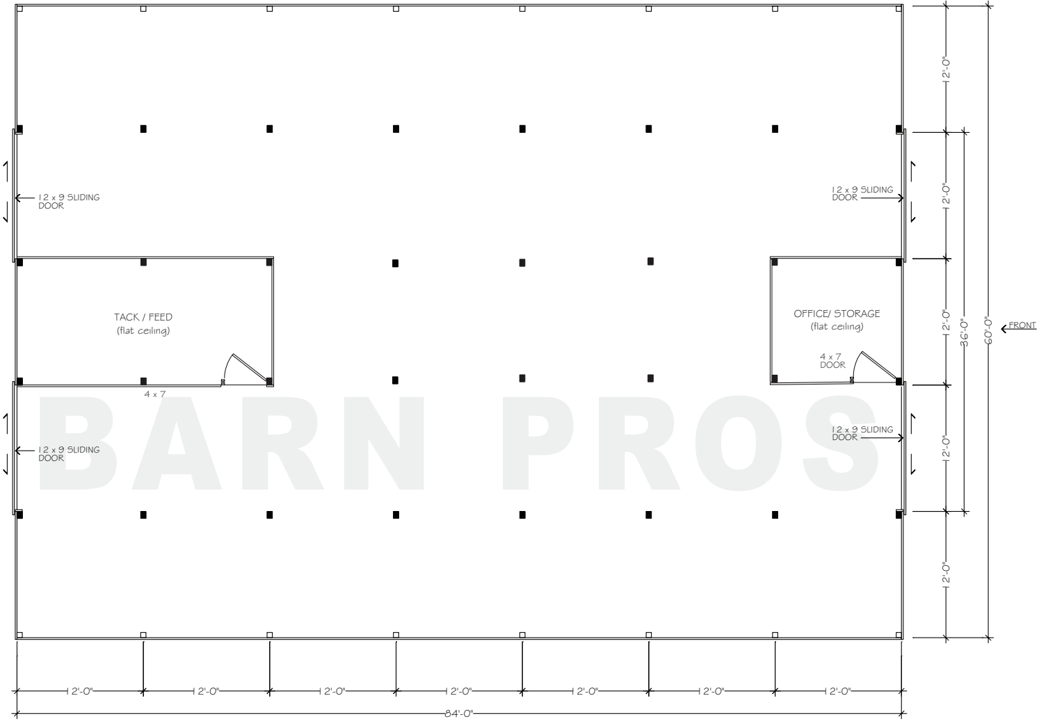
FLOORPLAN - LOWER
