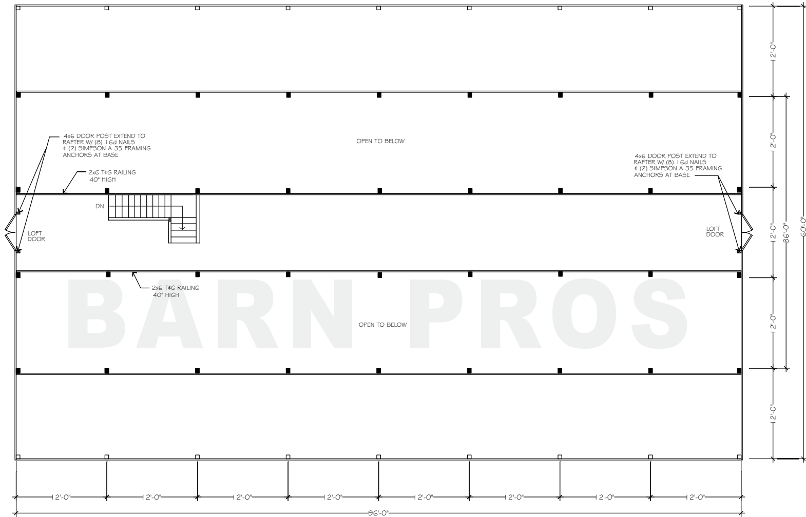
FLOORPLAN - UPPER
