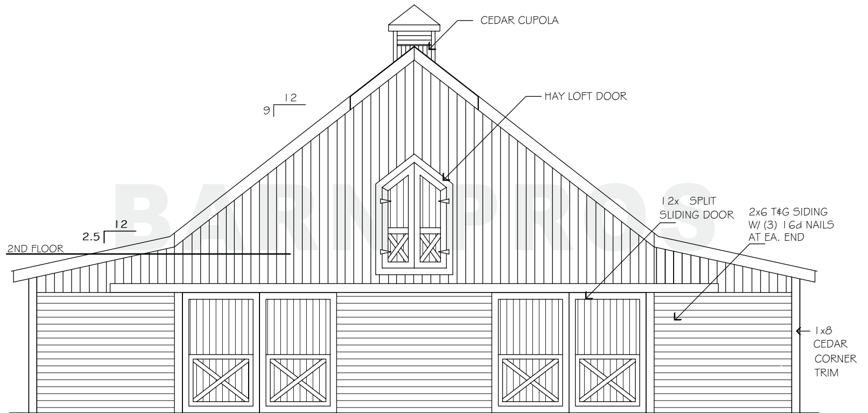
REAR ELEVATION
