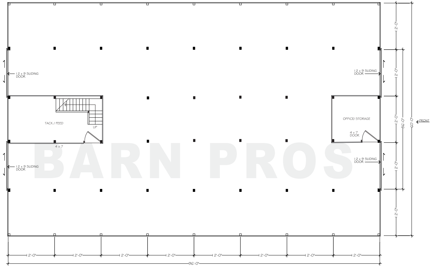
FLOORPLAN - LOWER
