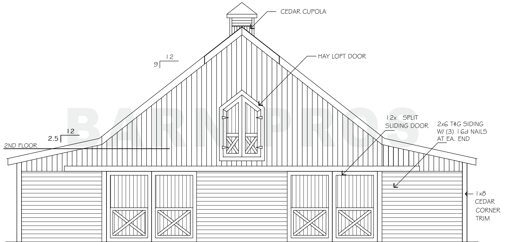
FRONT ELEVATION
