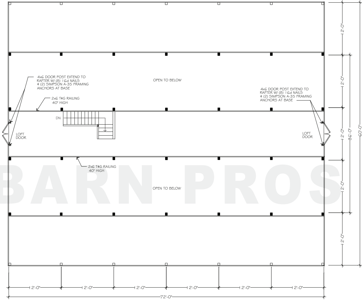
FLOORPLAN - UPPER
