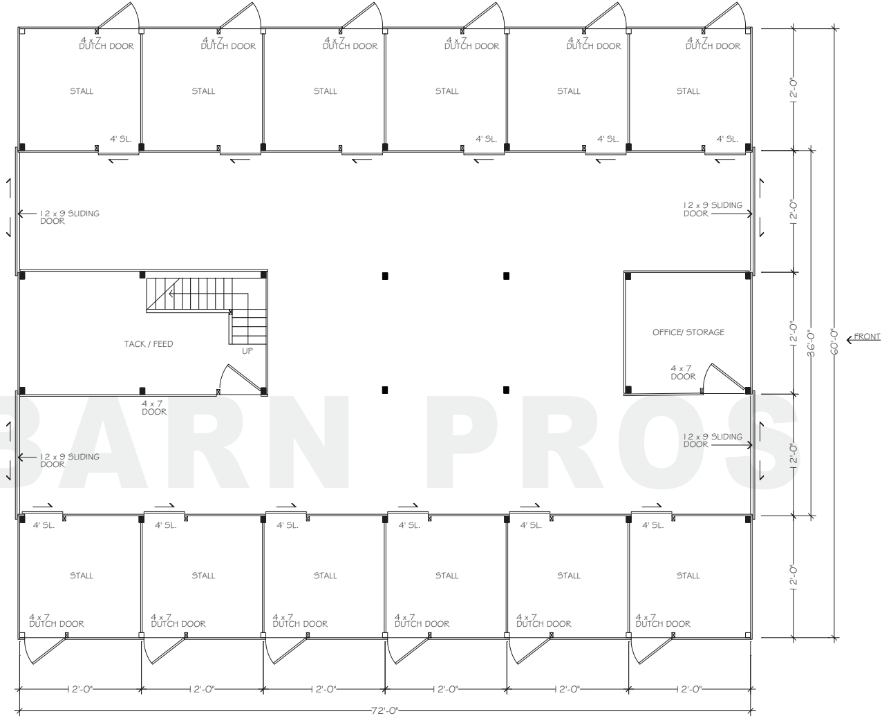
FLOORPLAN - LOWER
