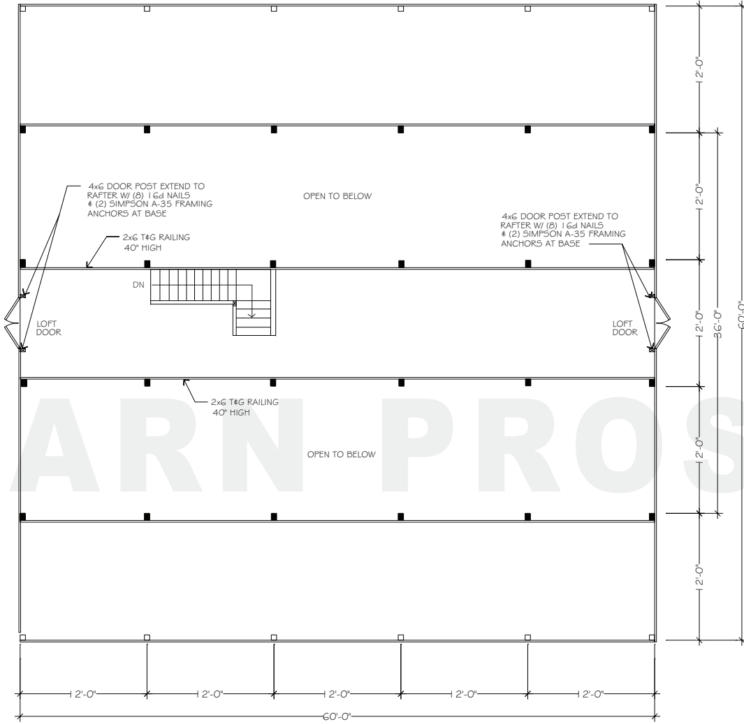
FLOORPLAN - UPPER
